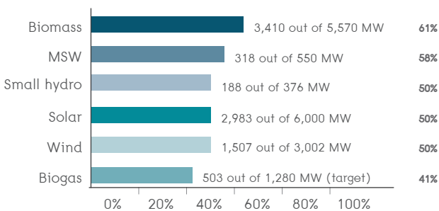
Figure : Renewable Energy Generation Capacity and AEDP* Target (as of 2019)
